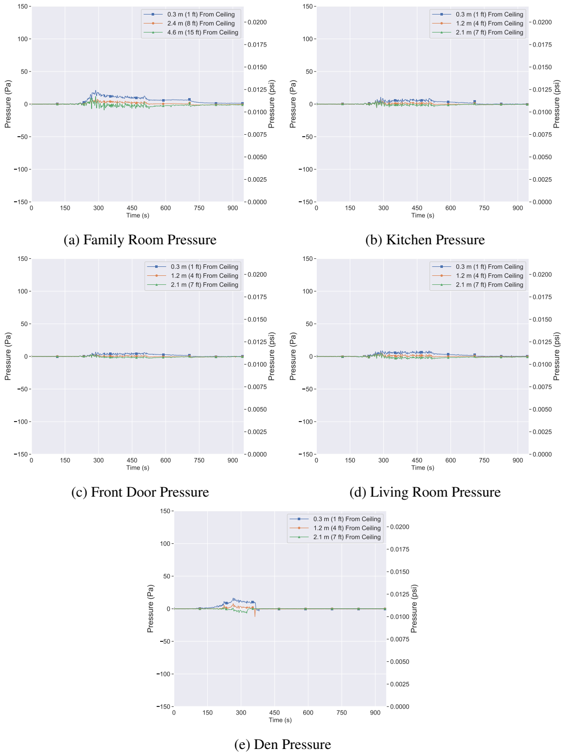
Figure 5.68: Experiment 7, front door and den window open, pressures in first floor rooms.
