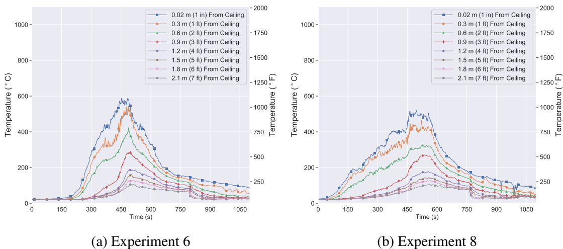
Figure 6.21: Comparison of closed door breakfast area temperatures.
